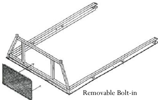
Basic Rack with Rear Carrier Assembly
