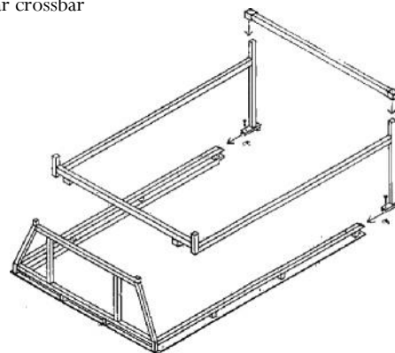
Contractor's Rack with removable rear crossbar (Exploded view)
